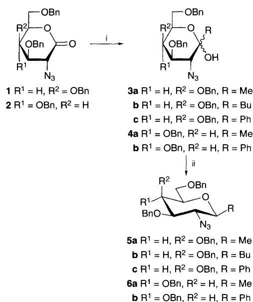
Scheme 1 Reagents and conditions: i, RLi (1.1 equiv.), toluene, -78^\circ\text{C} , 1 h; ii, Et 3 SiH (5 equiv.)–BF 3 ·Et 2 O (6 equiv.), MeCN, -40^\circ\text{C} , 15 min
